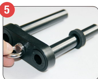
5 Place neoprene washers on to tubes, connect eyebolt and insert fitting into holes.
